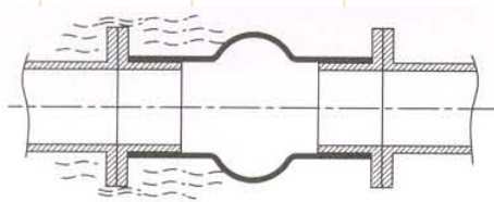
VIBRATION ISOLATION
