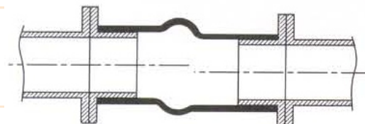
LATERAL DEFLECTION
