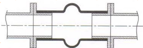
AXIAL CONTRACTION
